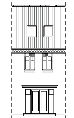
Back Elevation
